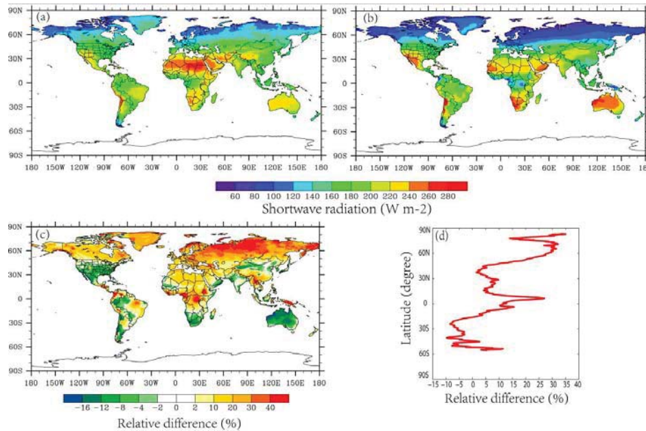
Fig. 1. The multi-model ensemble mean SW derived by VIC (a), and from ISI-MIP (b), relative difference between the VIC derived SW and the bias-corrected SW in the period of 1971-2009 (c) and the latitudinal profile of the difference (d).
