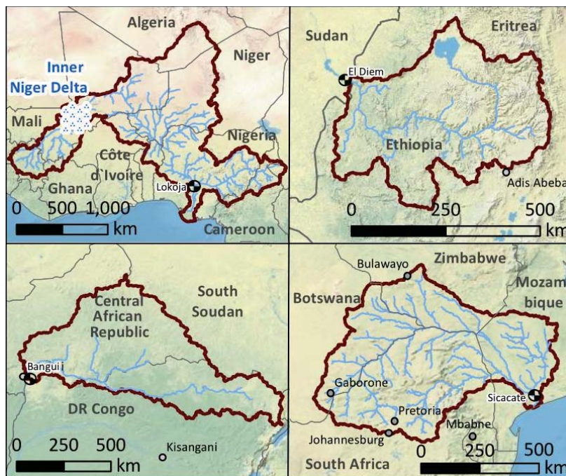
Figure 1 Map of the four modeled basins: Niger, Blue Nile, Ubangi, Limpopo (top left to bottom right).
